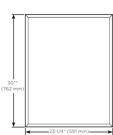
Cabinet Dimensions *Door is 1/8" (3 mm) smaller than cabinet
