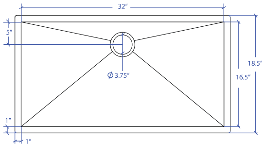
Under-mount
