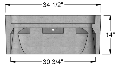
Shown: 68 PB-1PC Solid Concrete Cover With Bolt Down - 270 lbs
